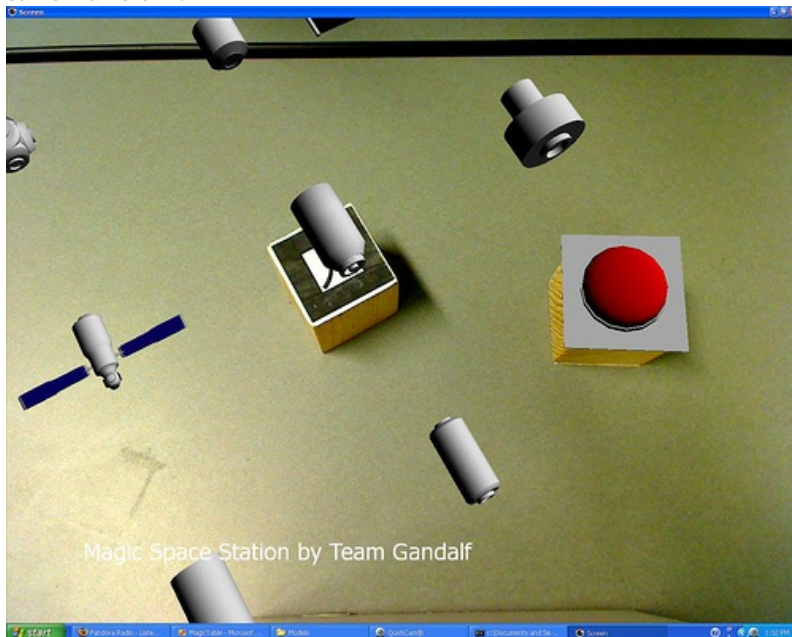
basic app
